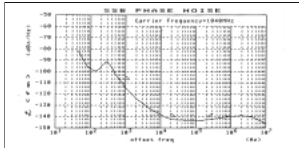
Fig. 1 SSB phase noise
