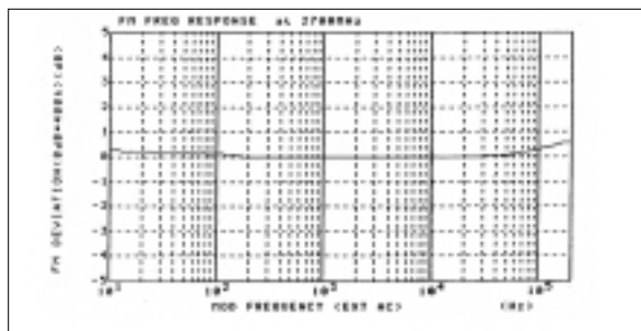
Fig. 5 FM modulation frequency characteristics
